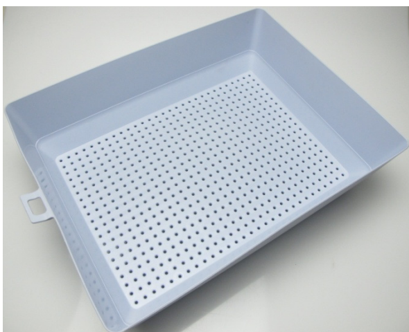
Photo 1: sieve (top view) after 40 autoclaving cycles
